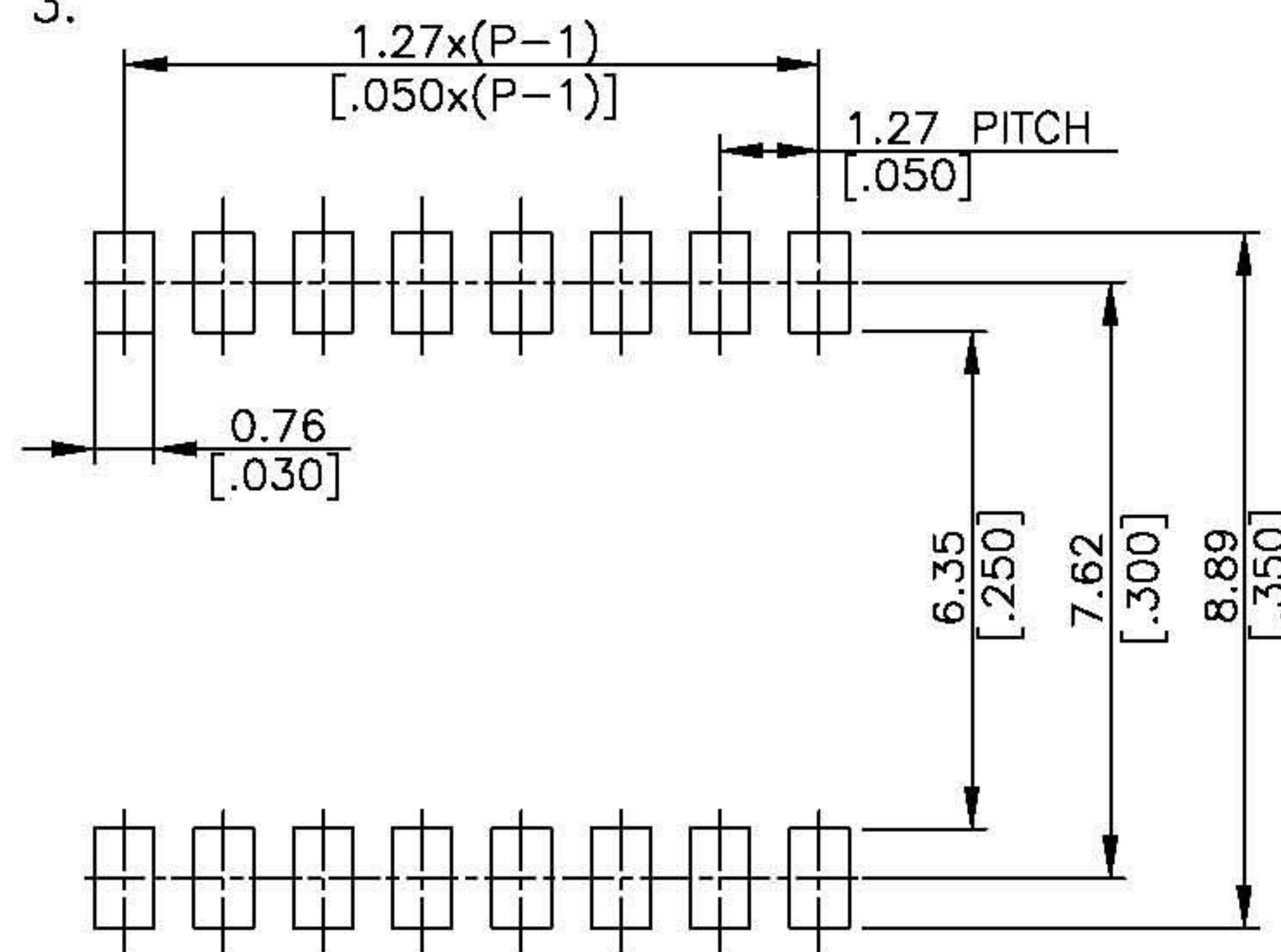
P. C. B LAYOUT
