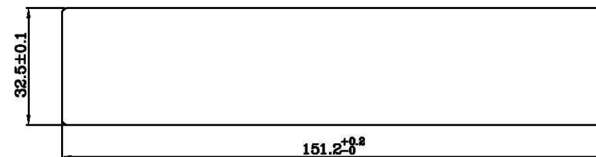
PANEL CUT-OUT
