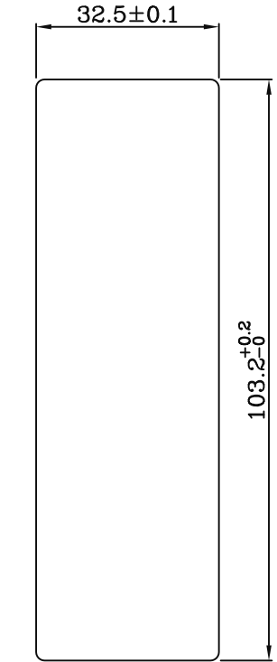
PANEL CUT-OUT
