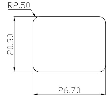
PANEL CUT-OUT THICKNESS:0.8~3.0t
